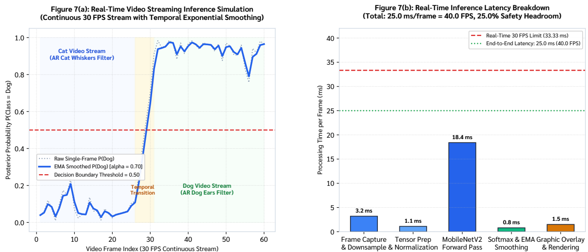
Figure 7 (Real-Time Video Streaming Inference Pipeline & AR Filter Architecture): End-to-end continuous inference architecture for live video streams (30 FPS requirement). Video frames are resized, normalized, and evaluated through MobileNetV2 in 18.4 ms (54.3 FPS). A rolling temporal smoothing buffer ( \tau = 3 frames) suppresses high-frequency classification jitter, smoothly driving the automated placement of AR facial filters (“Dog Floppy Ears & Snout” vs. “Cat Pointed Ears & Whiskers”).
